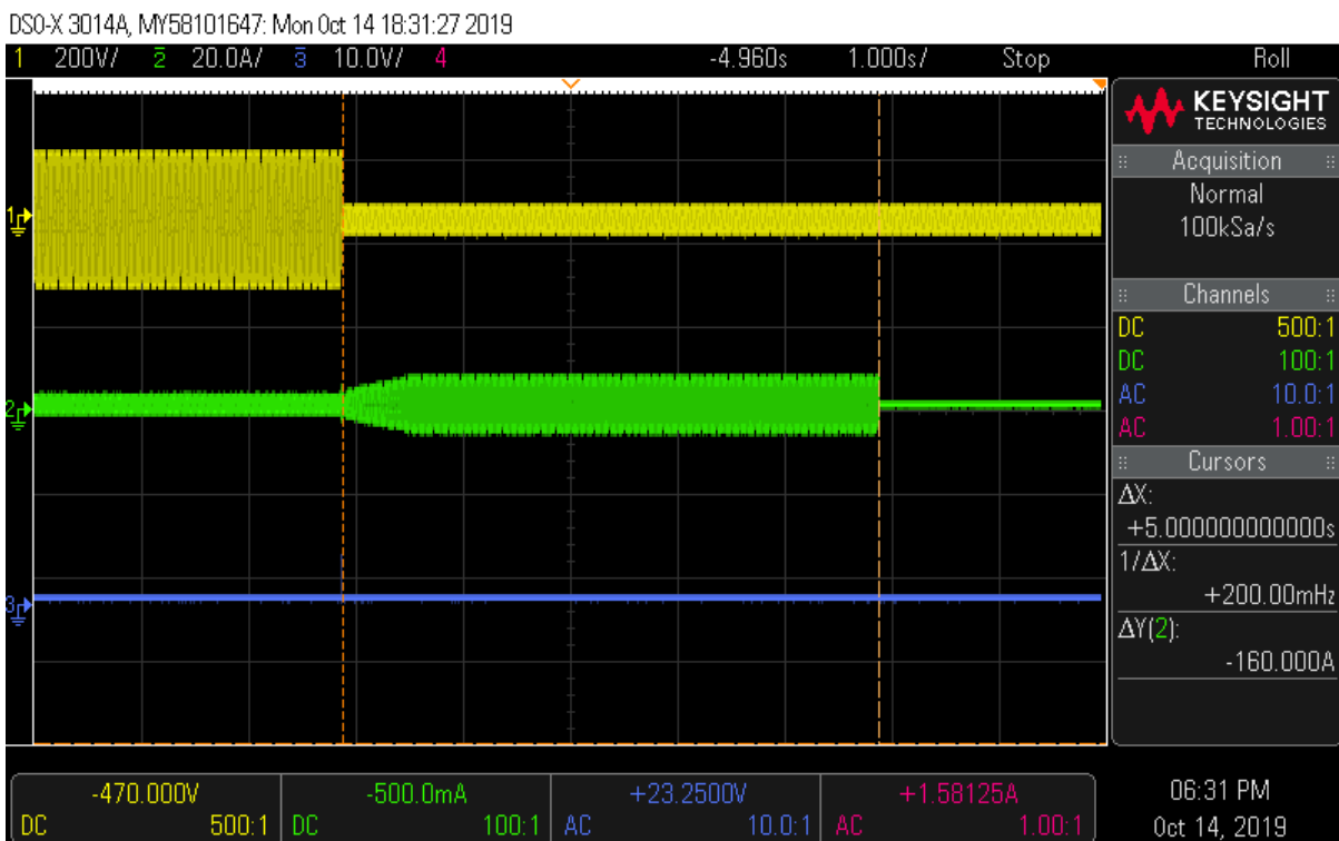
Trip time (5s setting)
