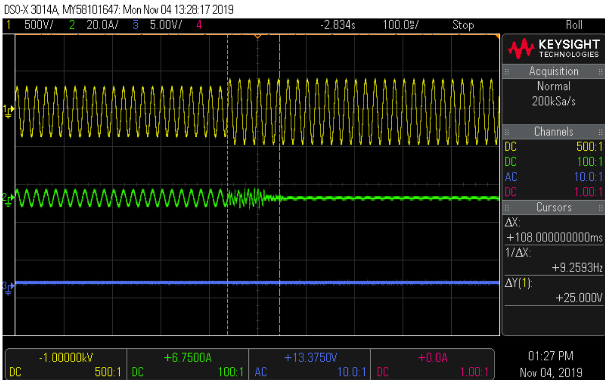
Trip time (0.1s setting)
