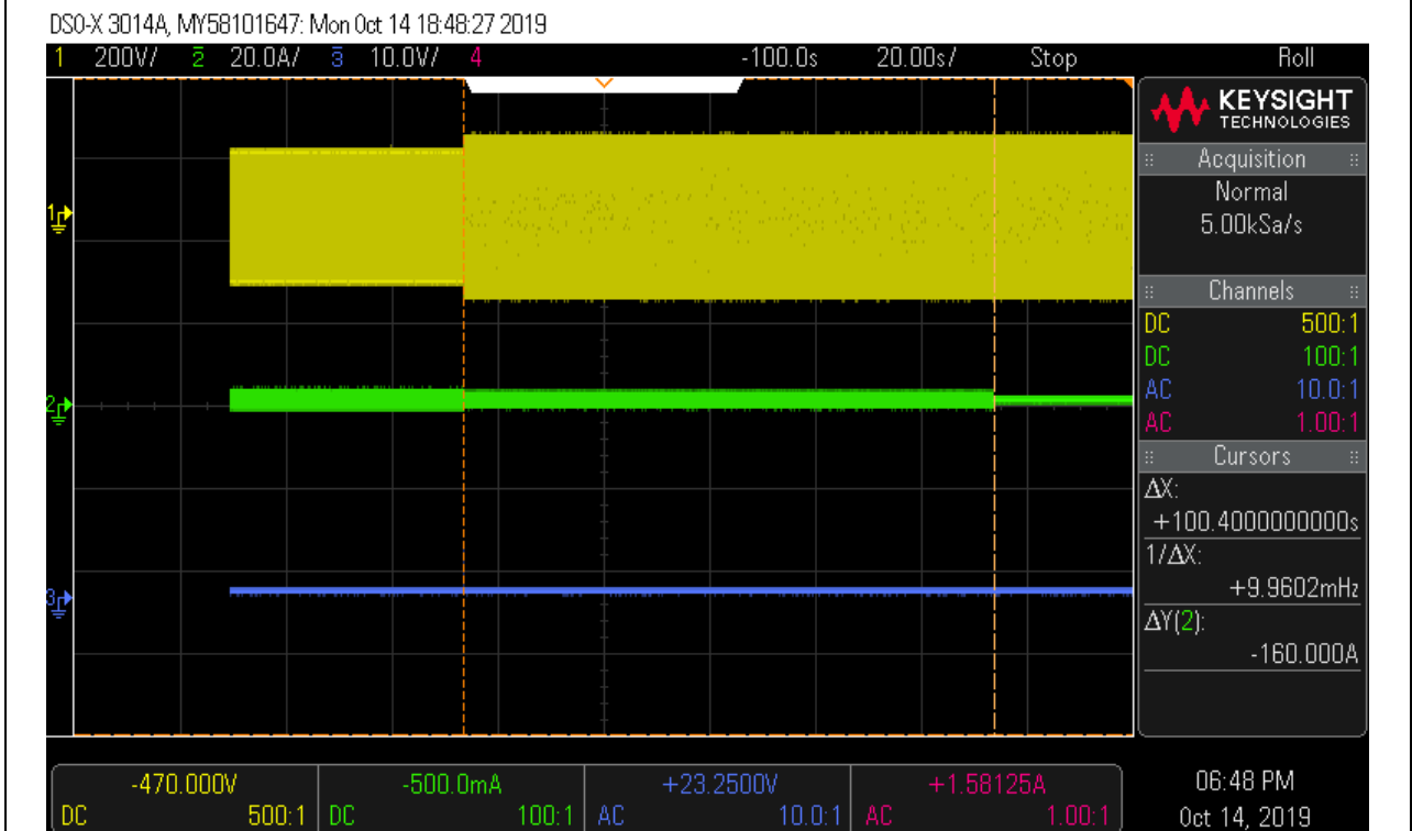
rip time (100s setting)
